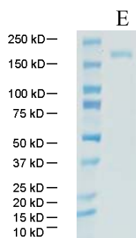
E: purified S (1-1190)(SARS-CoV) protein.
